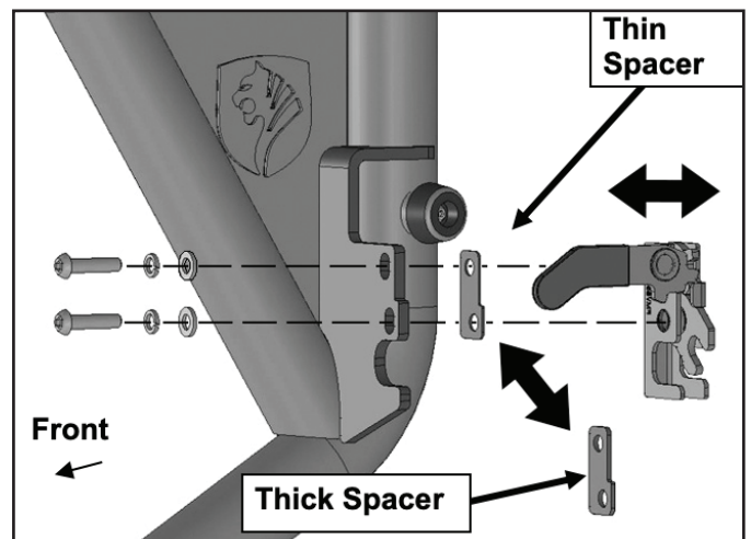
(Fig 9A) Use Thick, Thin or both 2-Hole Spacers if necessary, to line up Latch with striker
