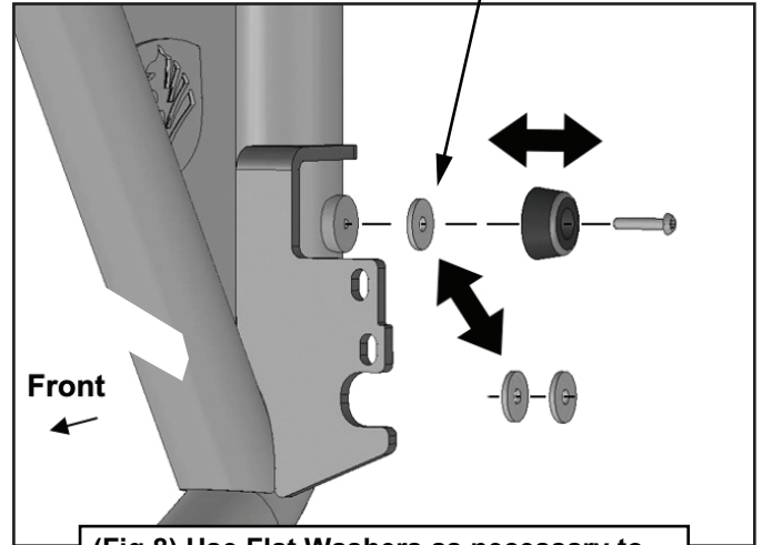
(Fig 8) Use Flat Washers as necessary to adjust fit of Door and Door Latch to vehicle
