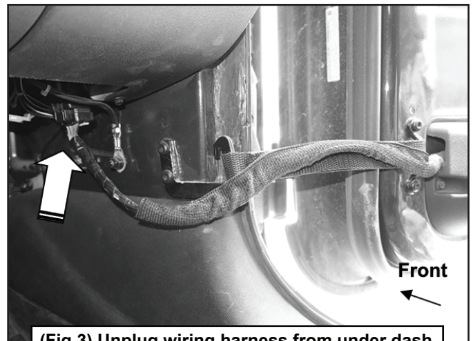
(Fig 3) Unplug wiring harness from under dash if equipped, (arrow). Release door stop strap
