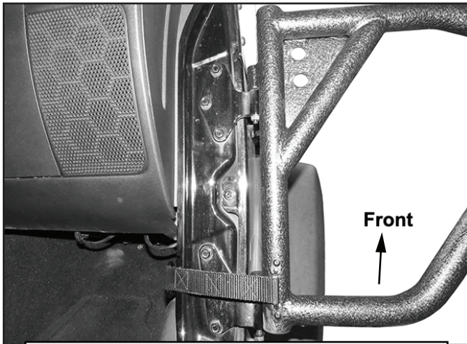
(Fig 7) Slide end of Door Stop Strap over bracket
