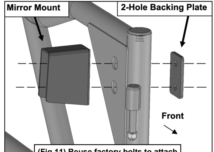
(Fig 11) Reuse factory bolts to attach outside mirror to Mount and Door
