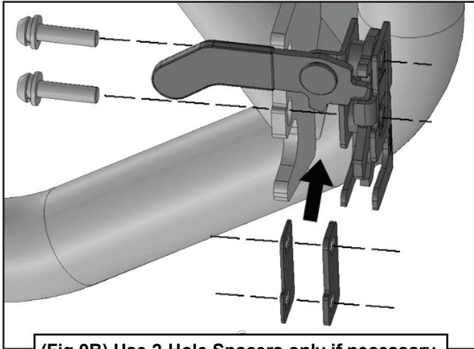
(Fig 9B) Use 2-Hole Spacers only if necessary, to line up Latch with striker
